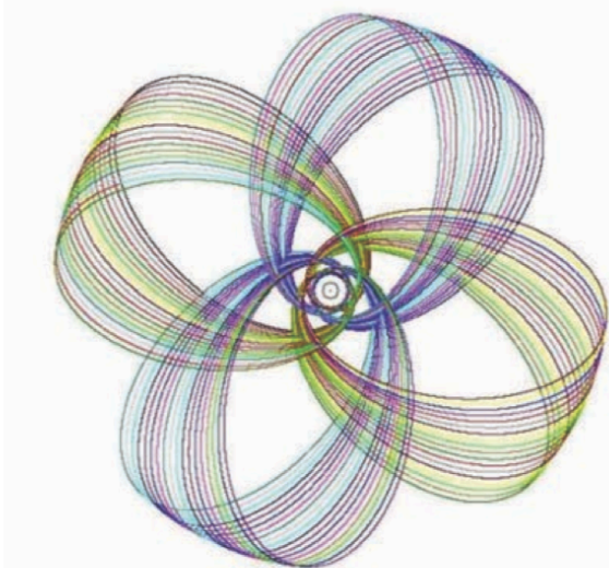
Fig.1 Nonlinear zoom-whirl orbits, color coded for each pass.
