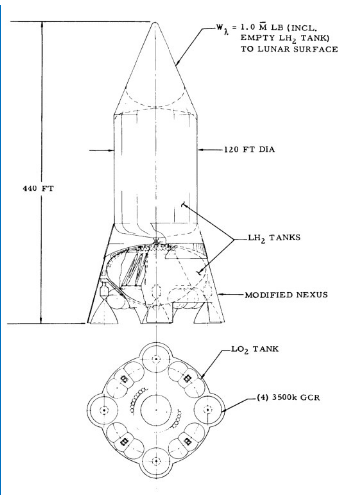
Above: Design P/S-E-LV 3.5, the "Super NEXUS." (Convair) Image credit: Scott Lowther.
