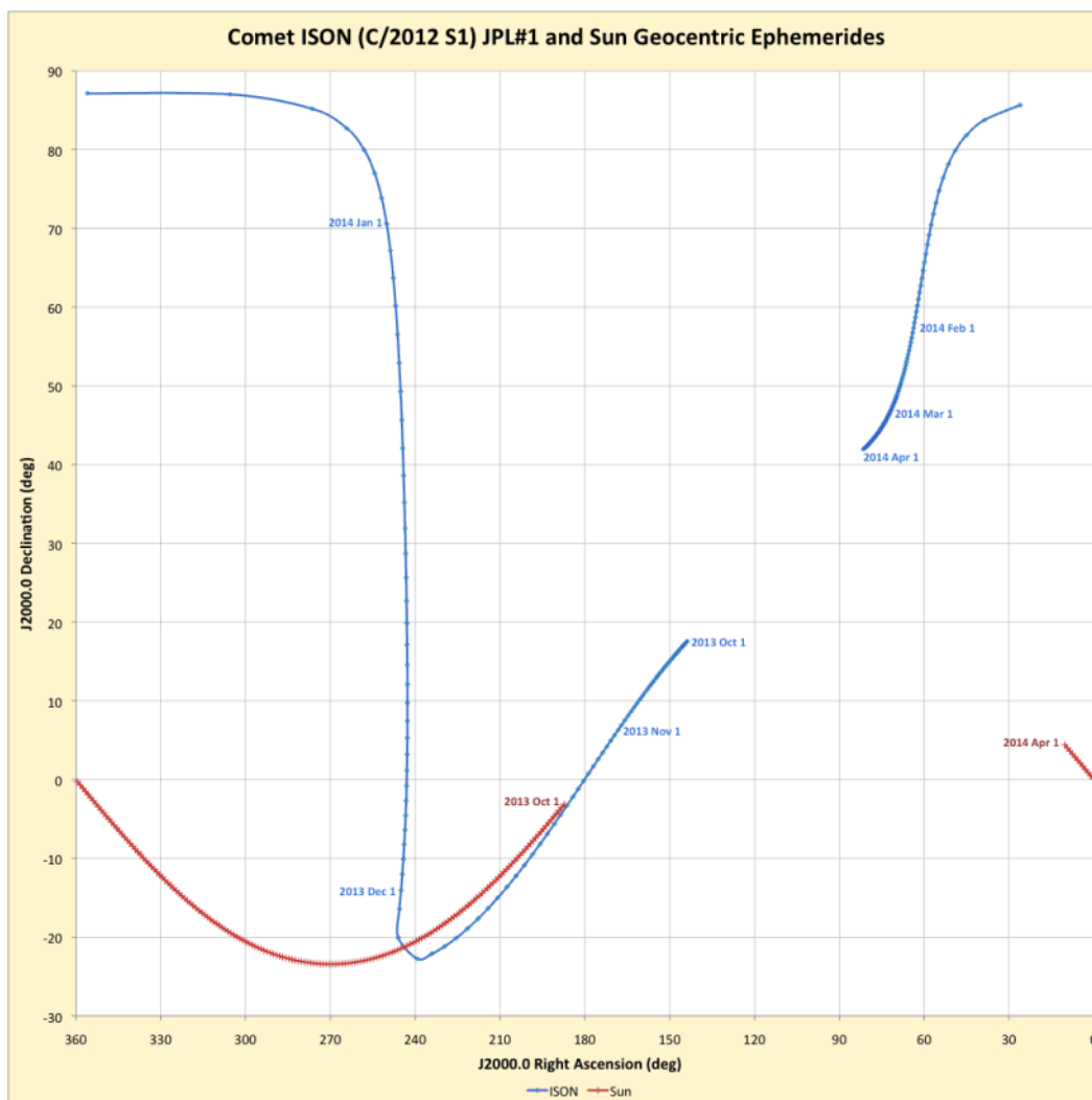
Figure 2. The apparent paths of ISON (blue) and the Sun (russet) are plotted from 2013 October 1 to 2014 April 1 on the geocentric celestial sphere's interior (east is left and north is up). Note the Sun's path coincides with a sector of the ecliptic plane projected onto this sphere. Prior to perihelion in late November, ISON will be visible to earthbound observers above the eastern horizon before sunrise. After perihelion, ISON rapidly moves north to become circumpolar at U.S. latitudes by late December 2013. As ISON moves south in early 2014, it enters the evening sky to become visible above the western horizon after sunset.
